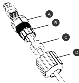
Figure 4: RJ-45 cable and cable gland assembly
