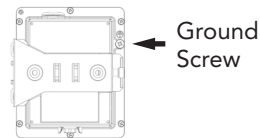
Figure 10: Connect good earth ground to AP here
